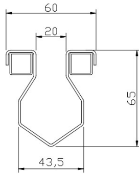
standard section
