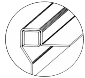
edge with reinforcement and flange for hydroisolation
