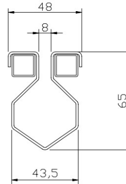
section with 8 mm gap for swimming pools and terraces
