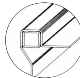
edge with reinforcement and flange for hydroisolation
